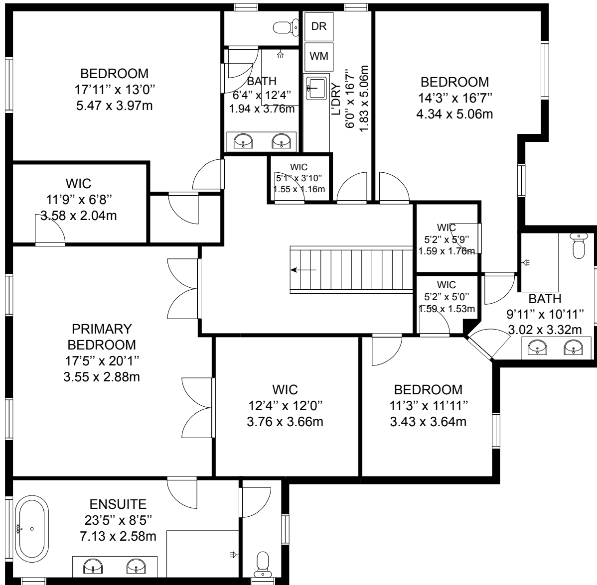
2ND FLOOR
